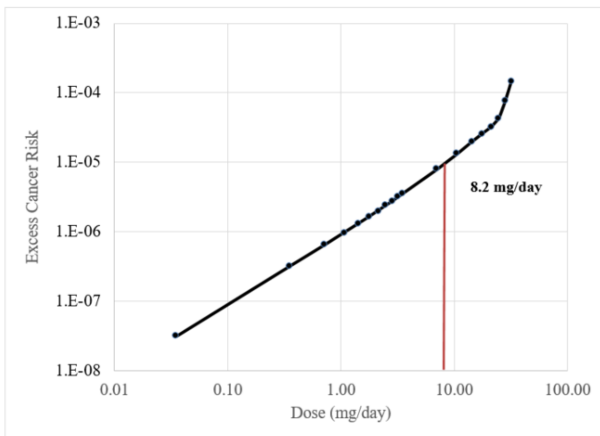
Figure 1. Dose-response model hockey stick-shaped model from (Ref. 12) representing mixed smokers and non-smokers. The dose (mg/day) was based on converting air concentration (ppm) to daily dose using ICH Q3C assumptions for human breathing volume (28,800 L/day).
